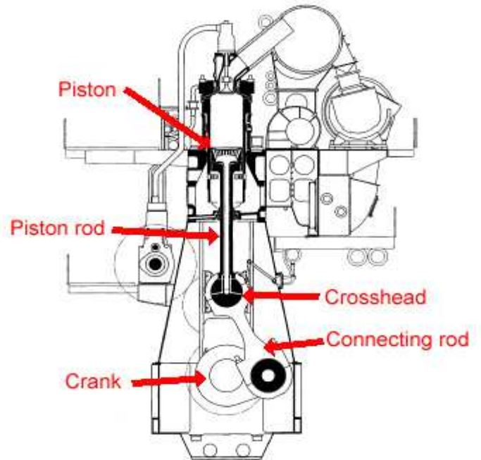
A cross section of the RTA96C
